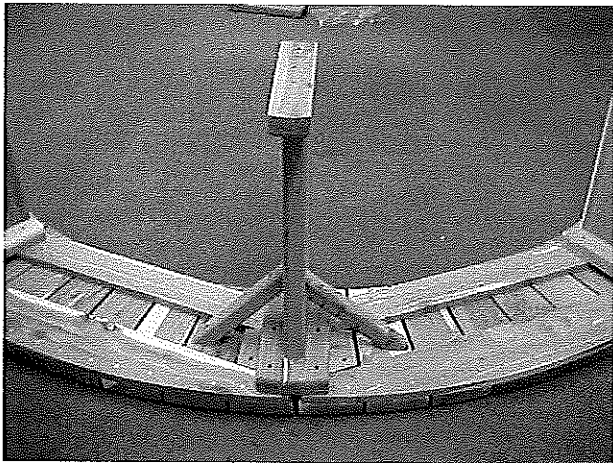
Center leg (2 braces)
